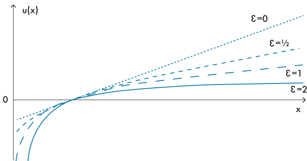
Figure A.3.4. Relationship between Utility and Income (x) for Different Values of \varepsilon
