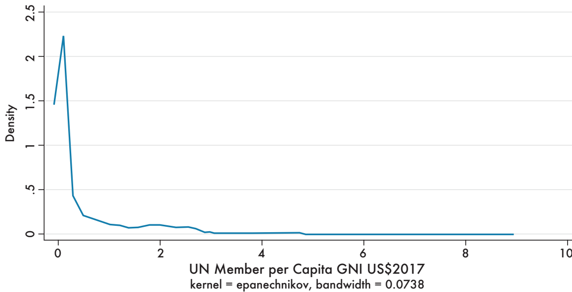
Figure A.1.7. Kernel Density Estimate of Member GNI per Capita
