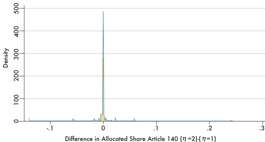
Figure A.2.50. Histogram and Kernel Density Estimator of (Difference in) Social Distribution Weights for the Original Formulae \eta=2 Minus Social Distribution Weights for the Original Formulae \eta=1 for Article 140 Shares
