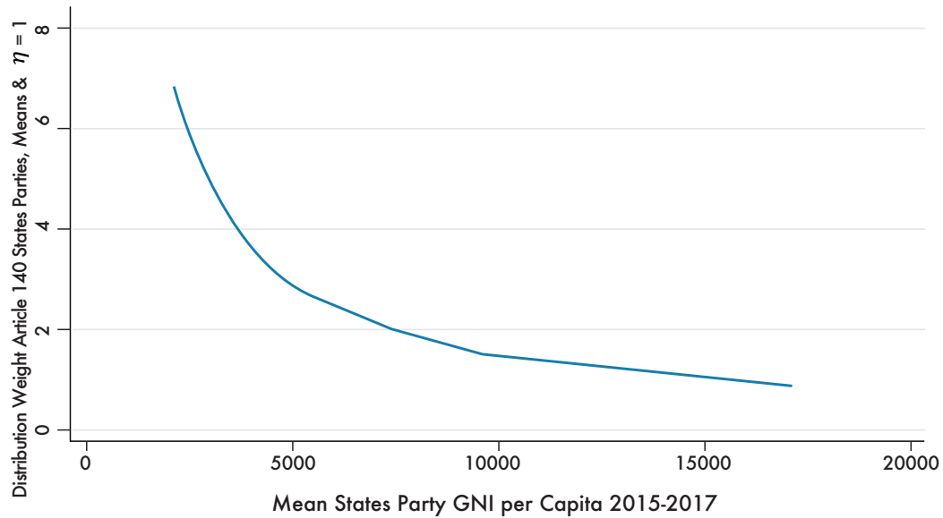
Figure A.2.9. Relationship between Distribution Weight \omega_i and State party per Capita GNI for Article 140 Distributions ( \eta=1 ): Western European and Others Group States parties
